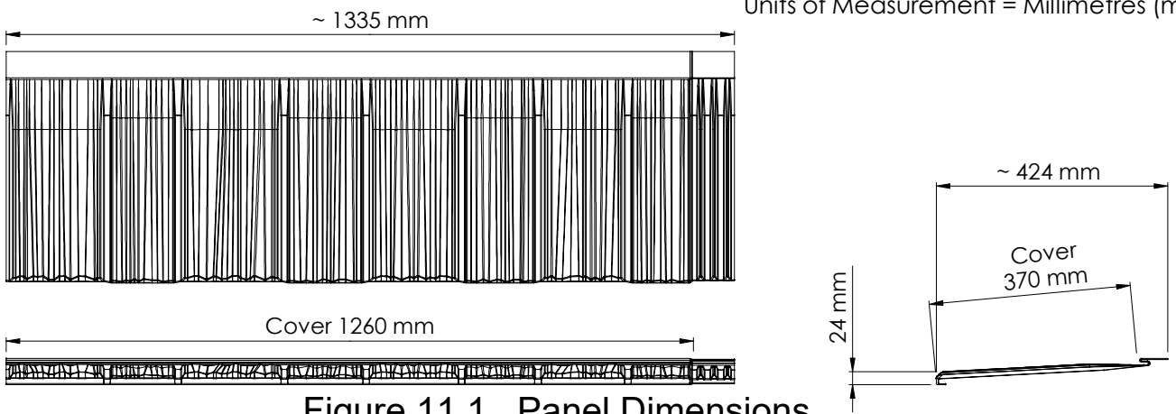
Figure 11.1 Panel Dimensions
