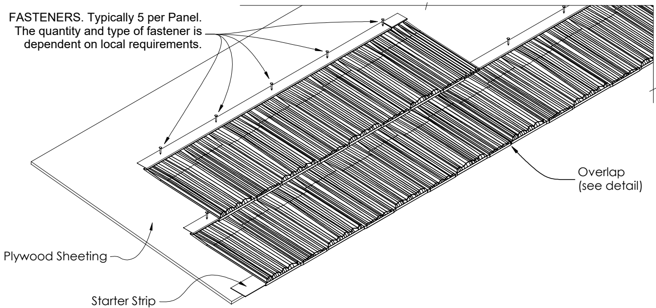
Figure 11.2 Fastening Detail
