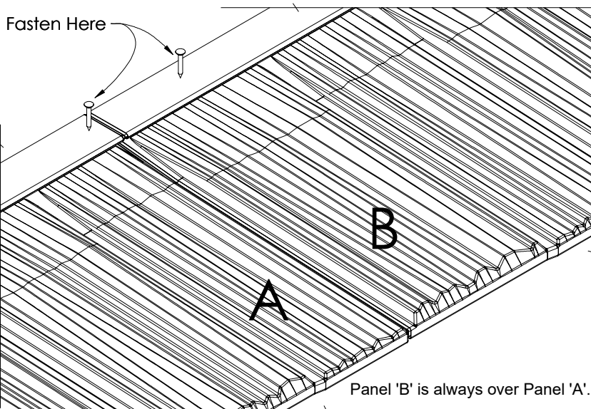
Figure 11.3 Overlap Detail
