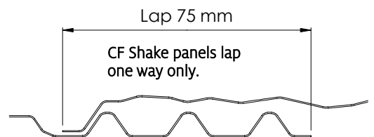
Figure 11.4 Side Lap Detail
