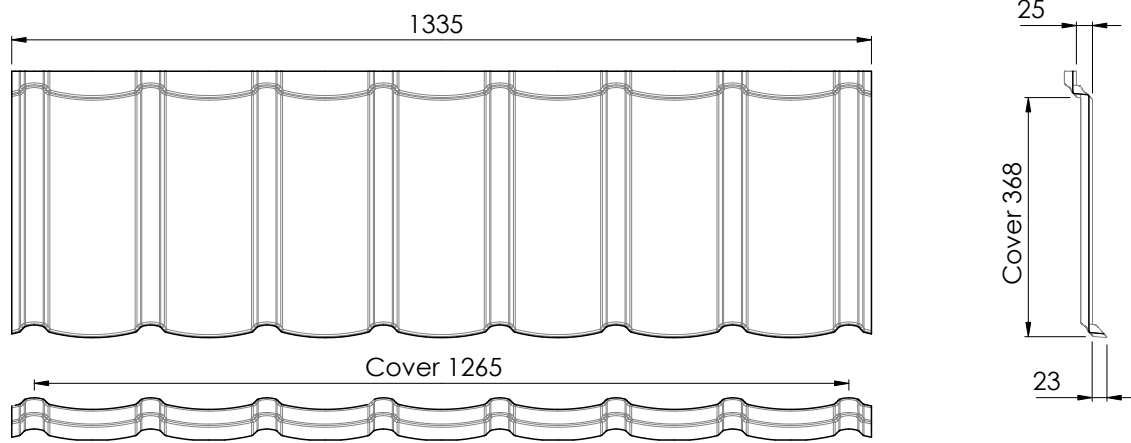
Figure 6.1 Tile Dimensions
