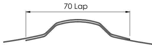
Figure 6.4 Lap Section
