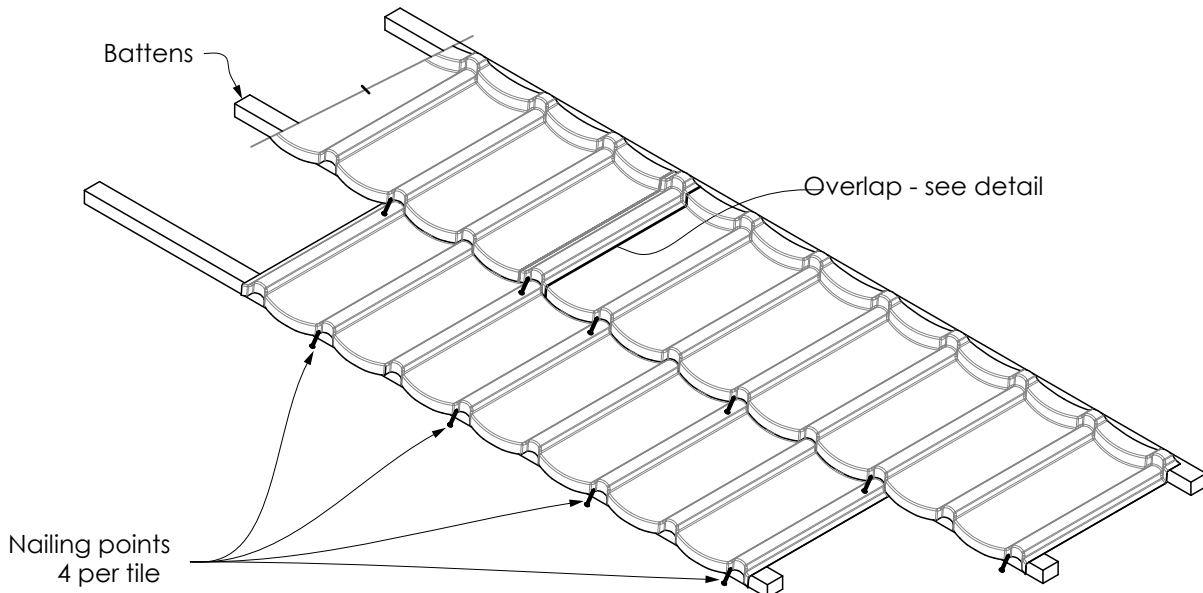
Figure 6.2 Nailing Detail
