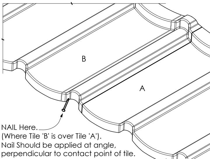
Figure 6.3 Overlap Detail
