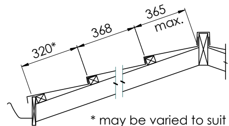
Figure 6.5 Batten Layout
