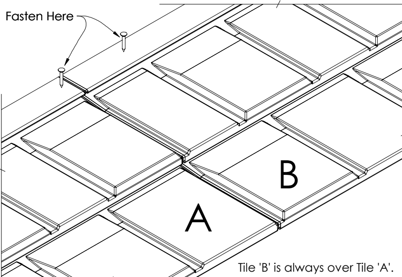
Figure 12.3 Overlap Detail
